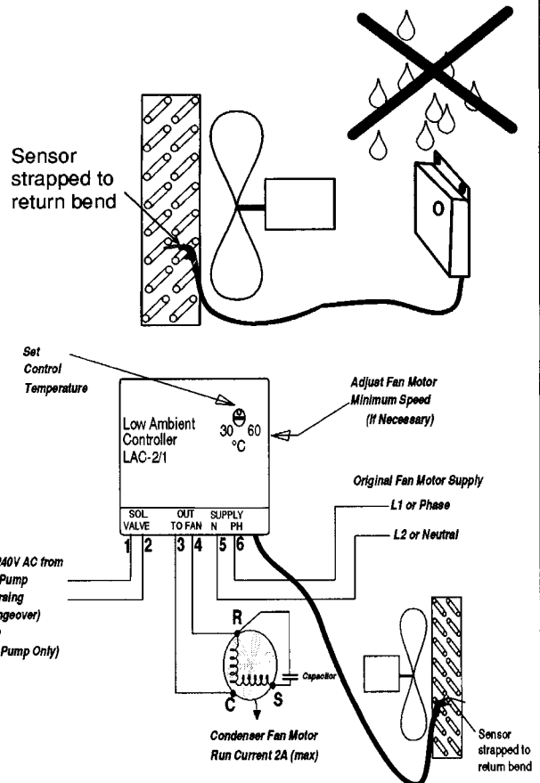
Standard Diagram For Wiring LAC-2/1 To Air Conditioner/Heat Pump Fan For Heat Pumps, add wiring to the Reversing (Changeover) Valve
